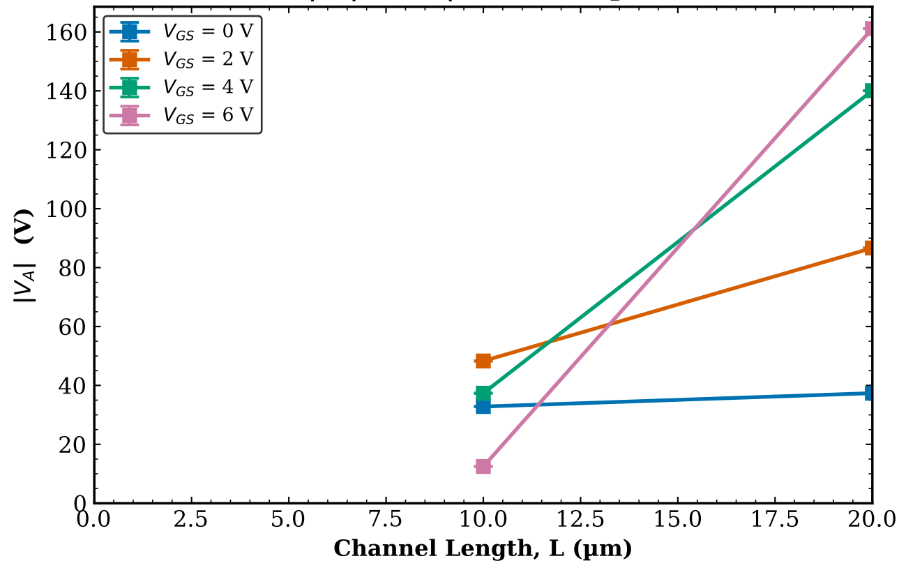
TFT1 Transistor 2 |V_A| vs L | W = 500\text{ }\mu\text{m}
